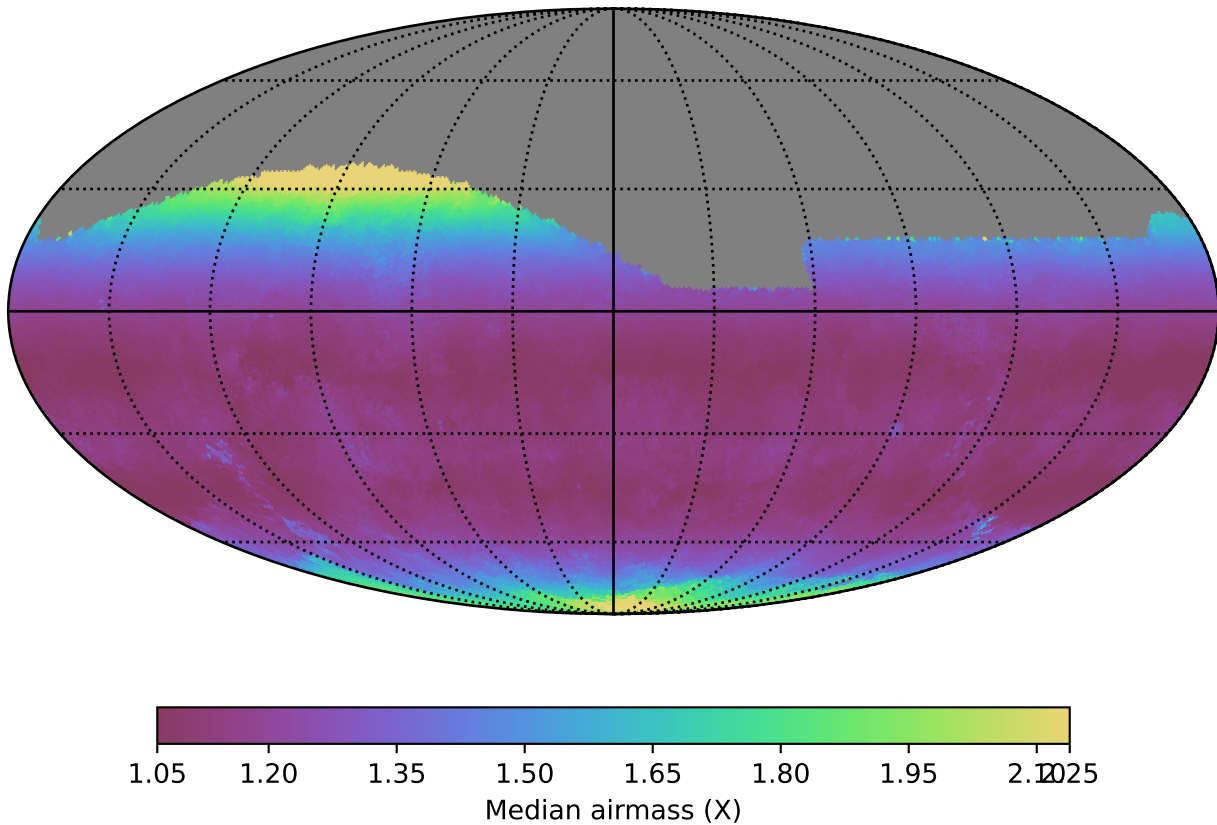
roman_v3.3_10yrs All sky g band: Median airmass
