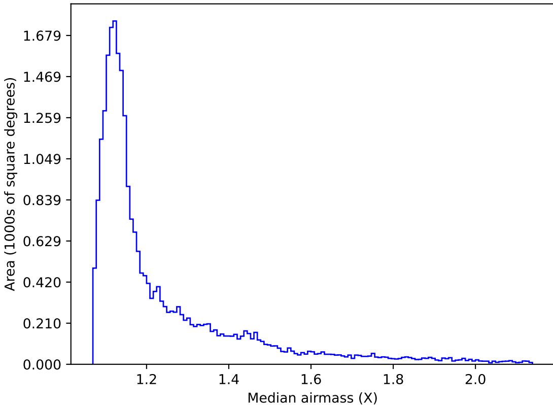
roman_v3.3_10yrs All sky g band: Median airmass
