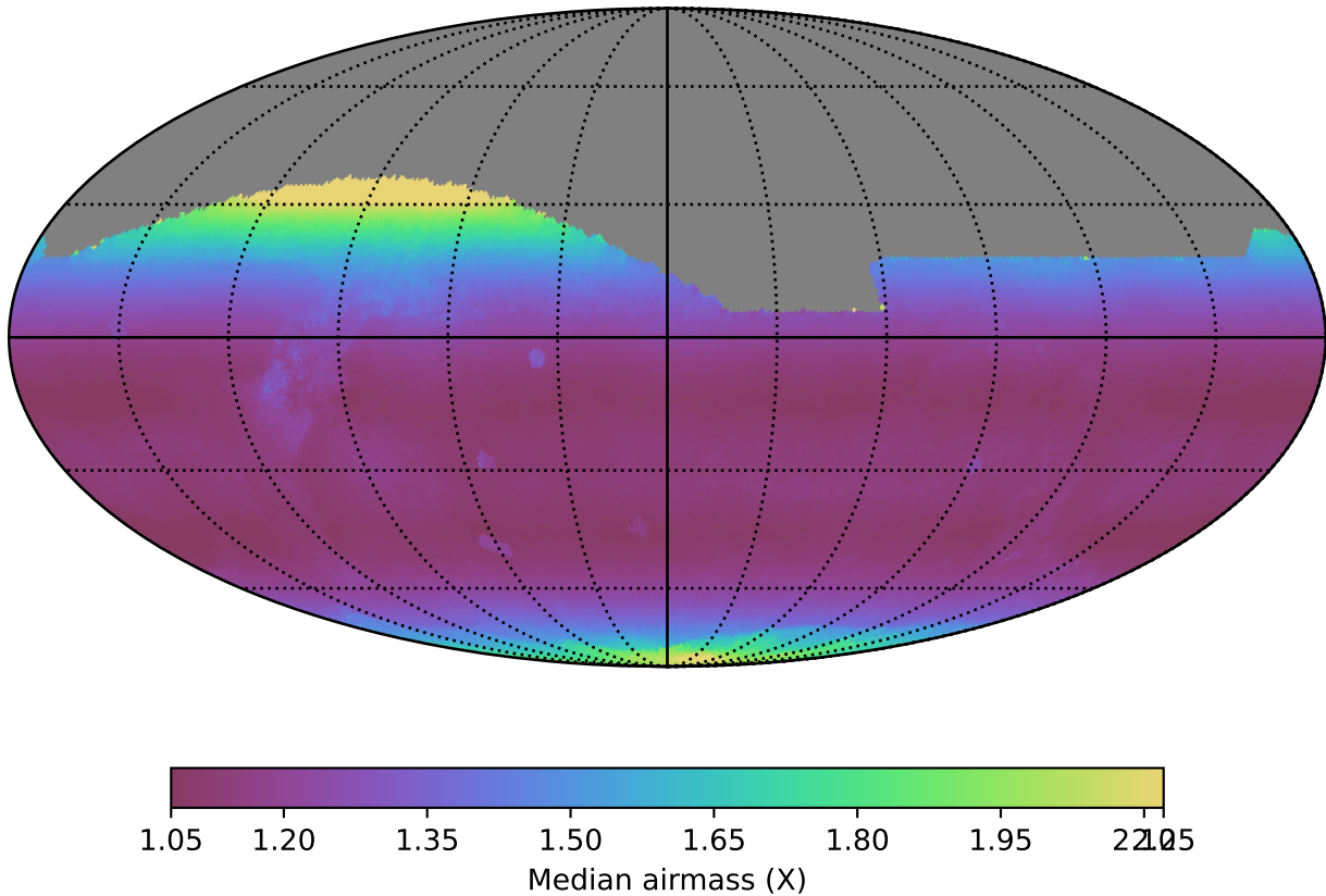
roman_v3.3_10yrs All sky all bands: Median airmass
