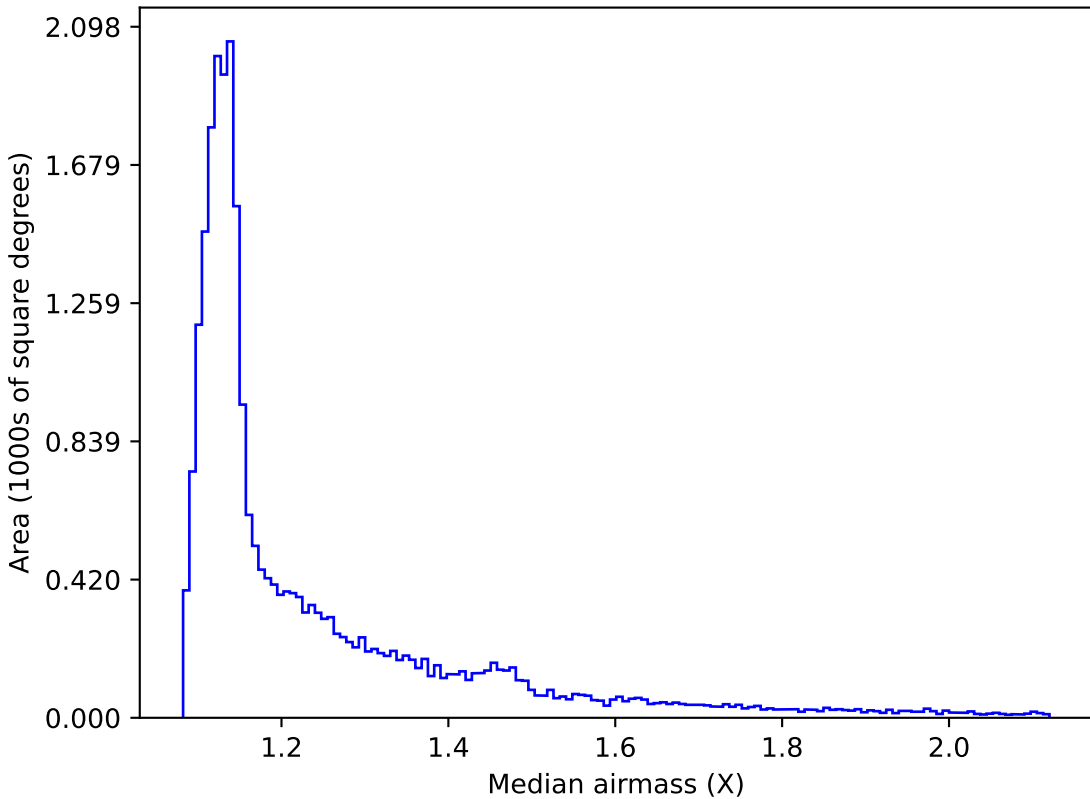
roman_v3.3_10yrs All sky all bands: Median airmass
