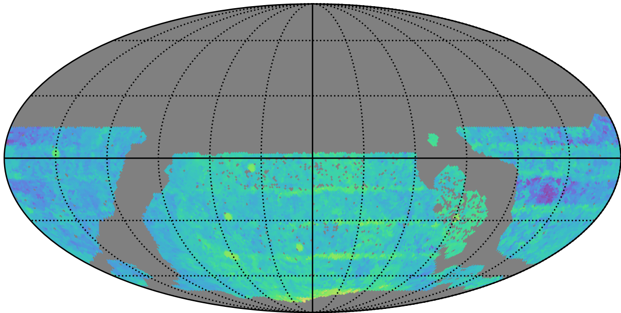
roman_v3.3_10yrs WFD z band: Median Season Length
