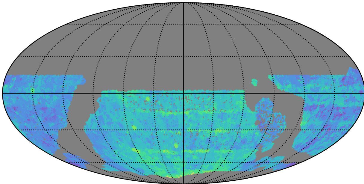
roman_v3.3_10yrs WFD y band: Median Season Length
