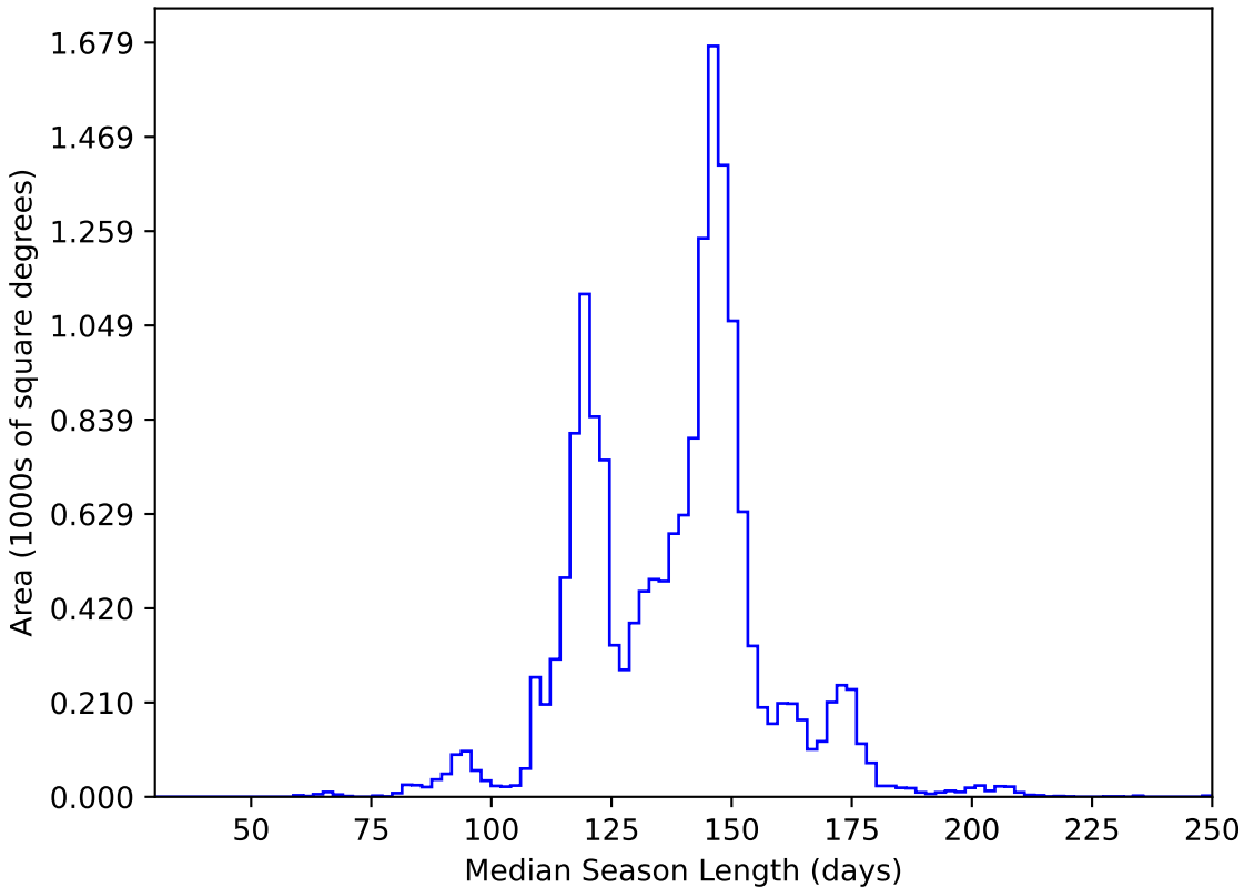
roman_v3.3_10yrs WFD y band: Median Season Length
