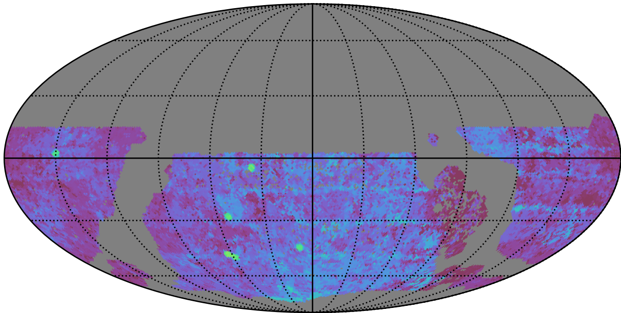
roman_v3.3_10yrs WFD u band: Median Season Length
