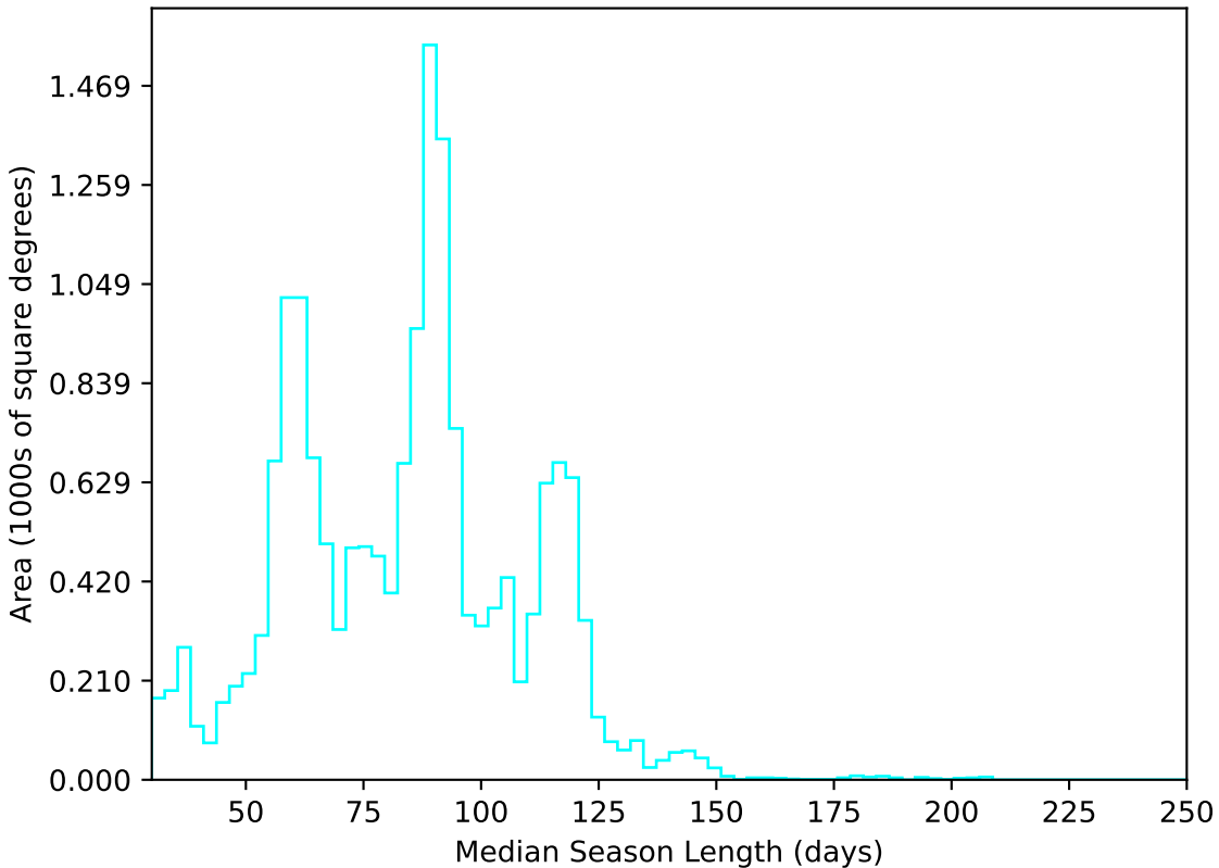
roman_v3.3_10yrs WFD u band: Median Season Length
