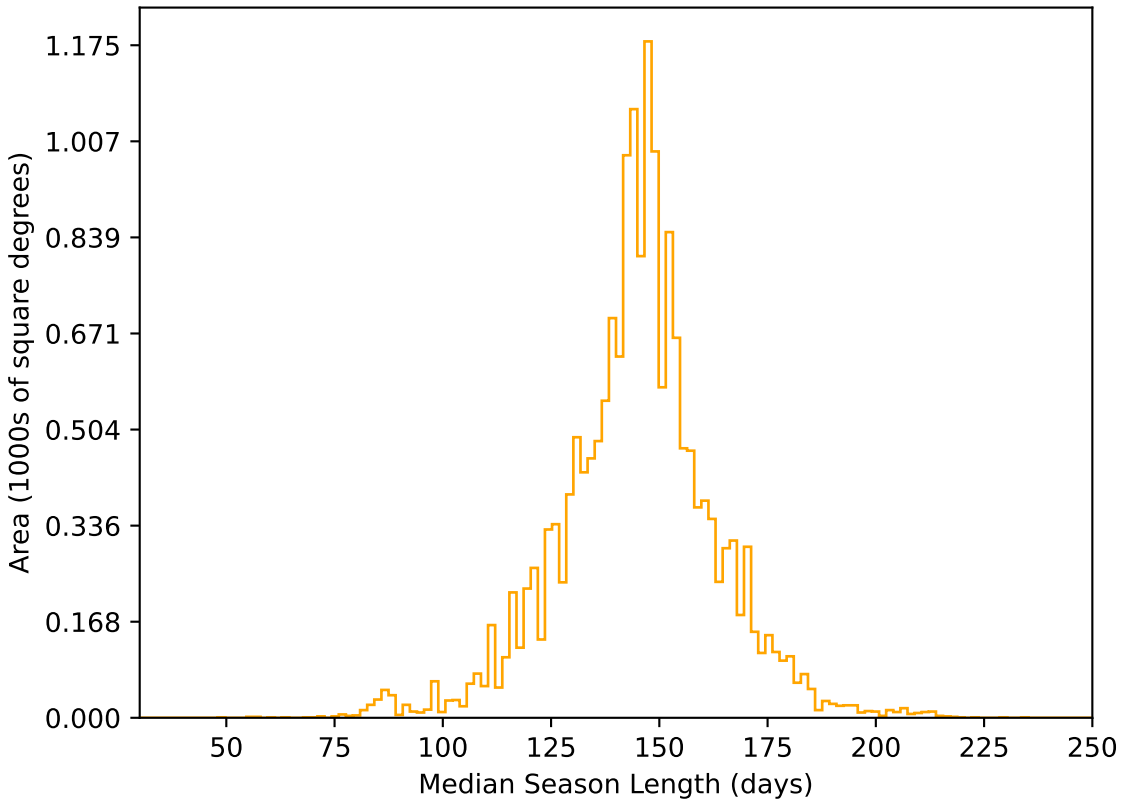
roman_v3.3_10yrs WFD r band: Median Season Length
