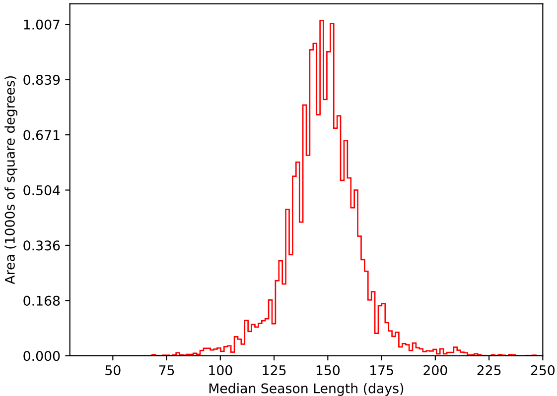
roman_v3.3_10yrs WFD i band: Median Season Length
