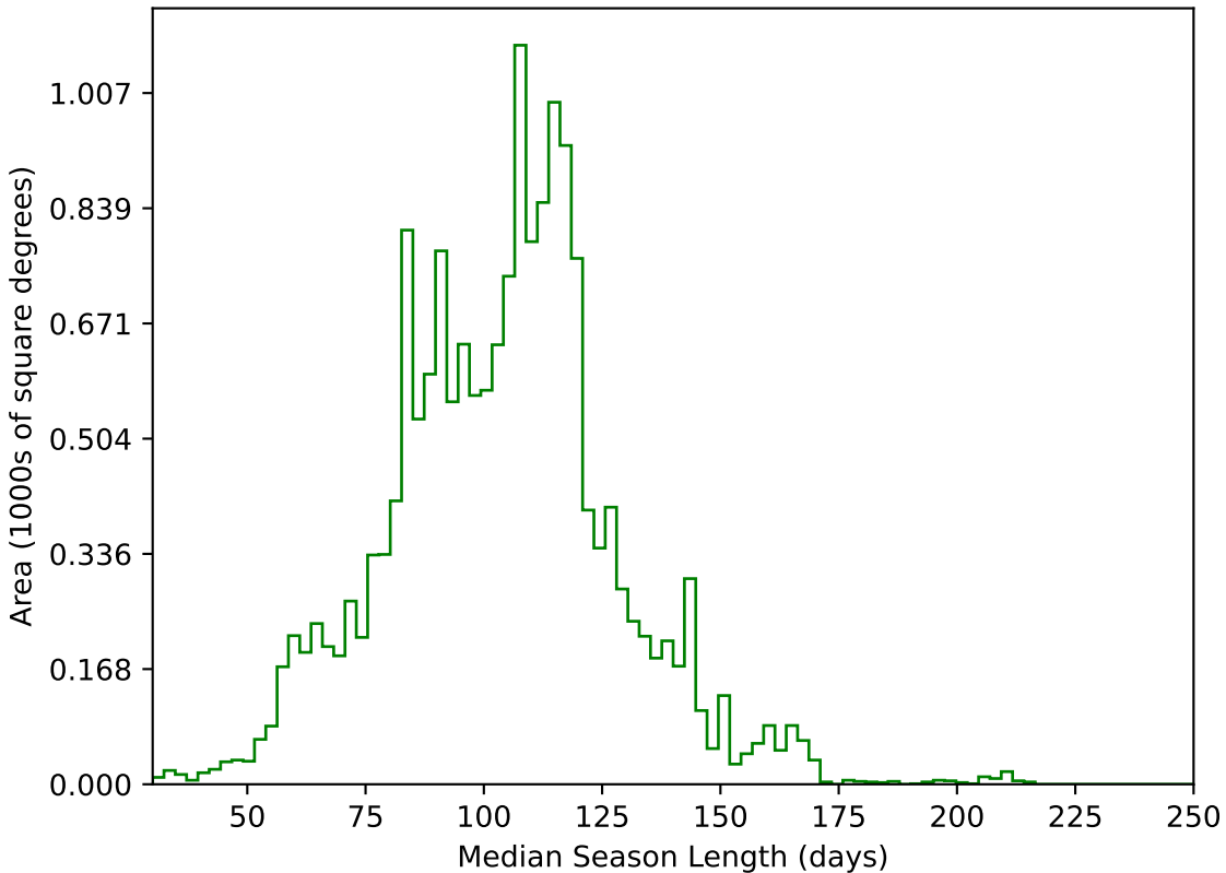
roman_v3.3_10yrs WFD g band: Median Season Length
