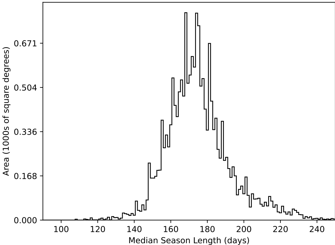
roman_v3.3_10yrs WFD all bands: Median Season Length
