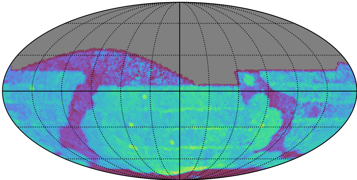
roman_v3.3_10yrs All sky z band: Median Season Length
