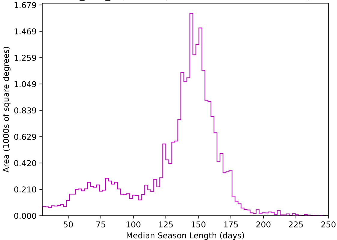
roman_v3.3_10yrs All sky z band: Median Season Length
