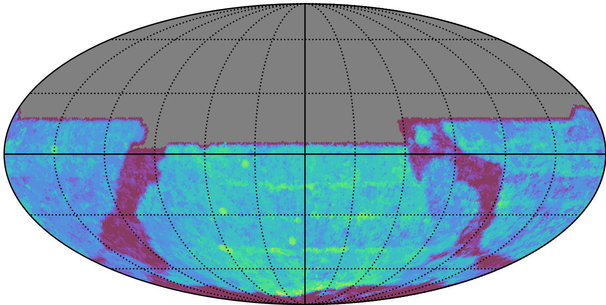
roman_v3.3_10yrs All sky y band: Median Season Length
