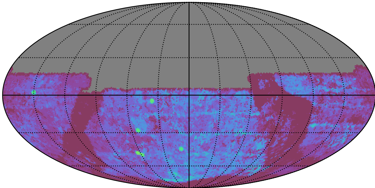
roman_v3.3_10yrs All sky u band: Median Season Length
