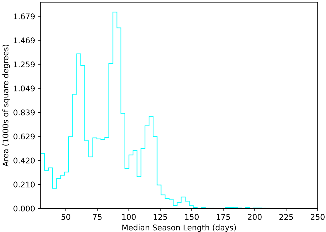
roman_v3.3_10yrs All sky u band: Median Season Length
