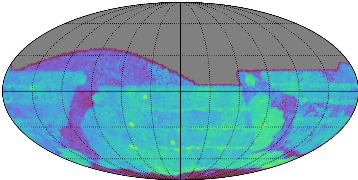
roman_v3.3_10yrs All sky r band: Median Season Length
