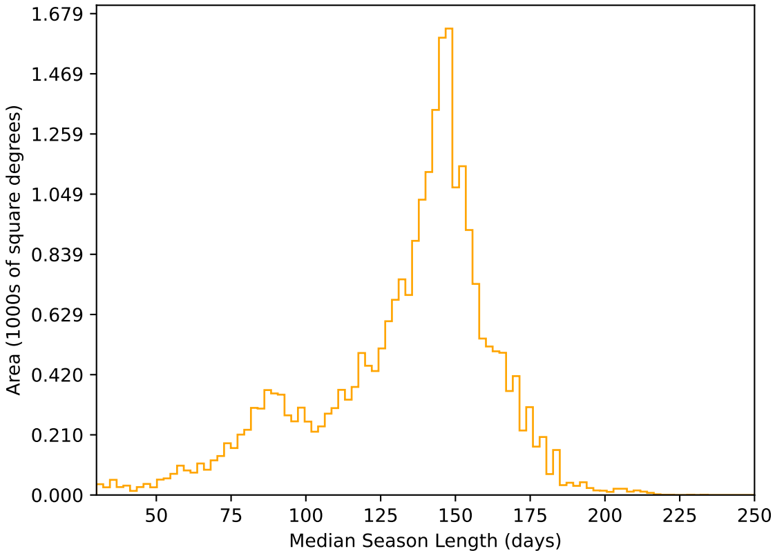
roman_v3.3_10yrs All sky r band: Median Season Length
