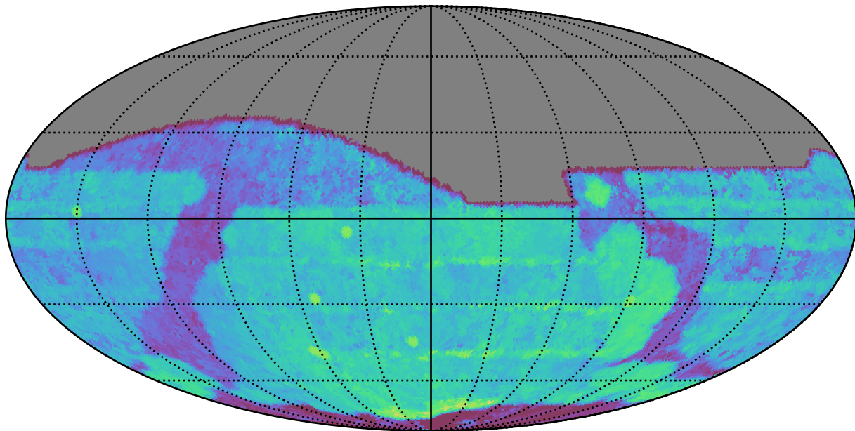
roman_v3.3_10yrs All sky i band: Median Season Length
