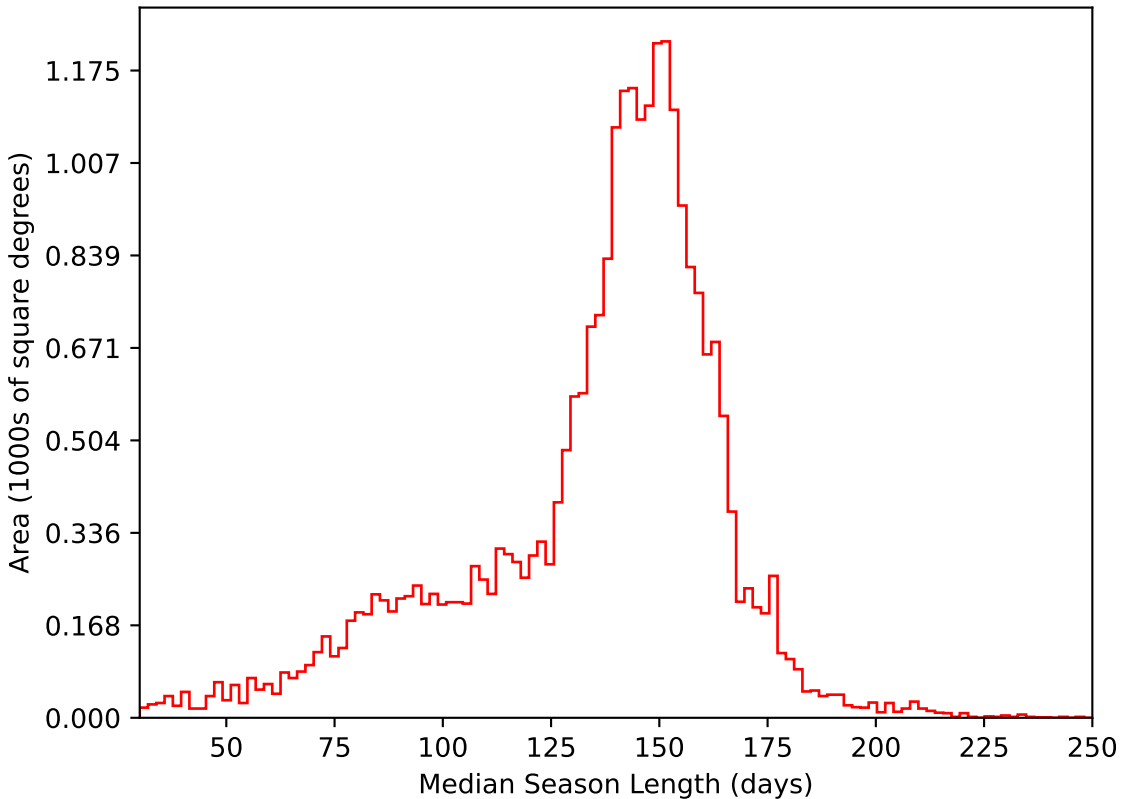
roman_v3.3_10yrs All sky i band: Median Season Length
