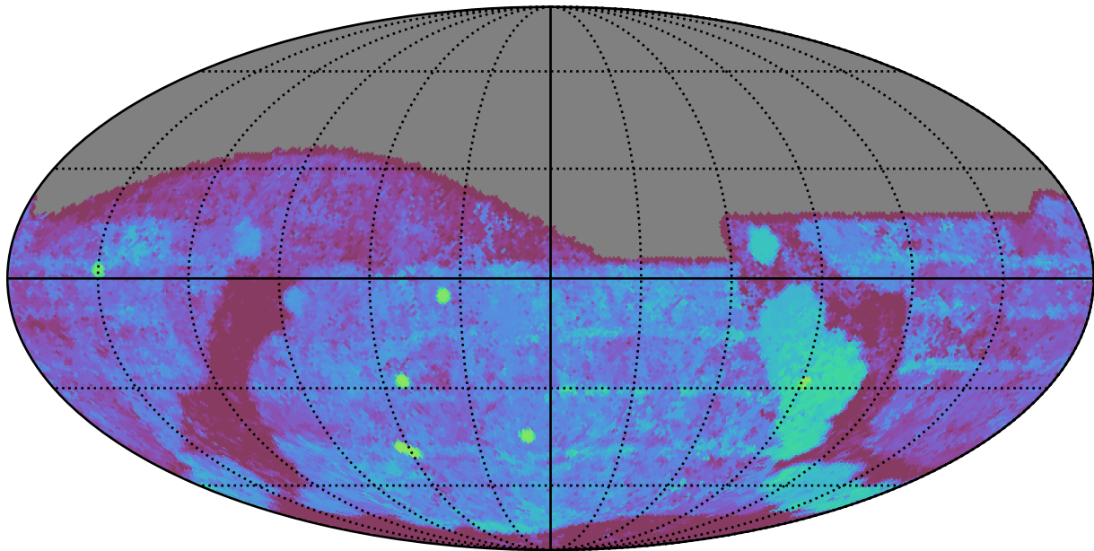
roman_v3.3_10yrs All sky g band: Median Season Length
