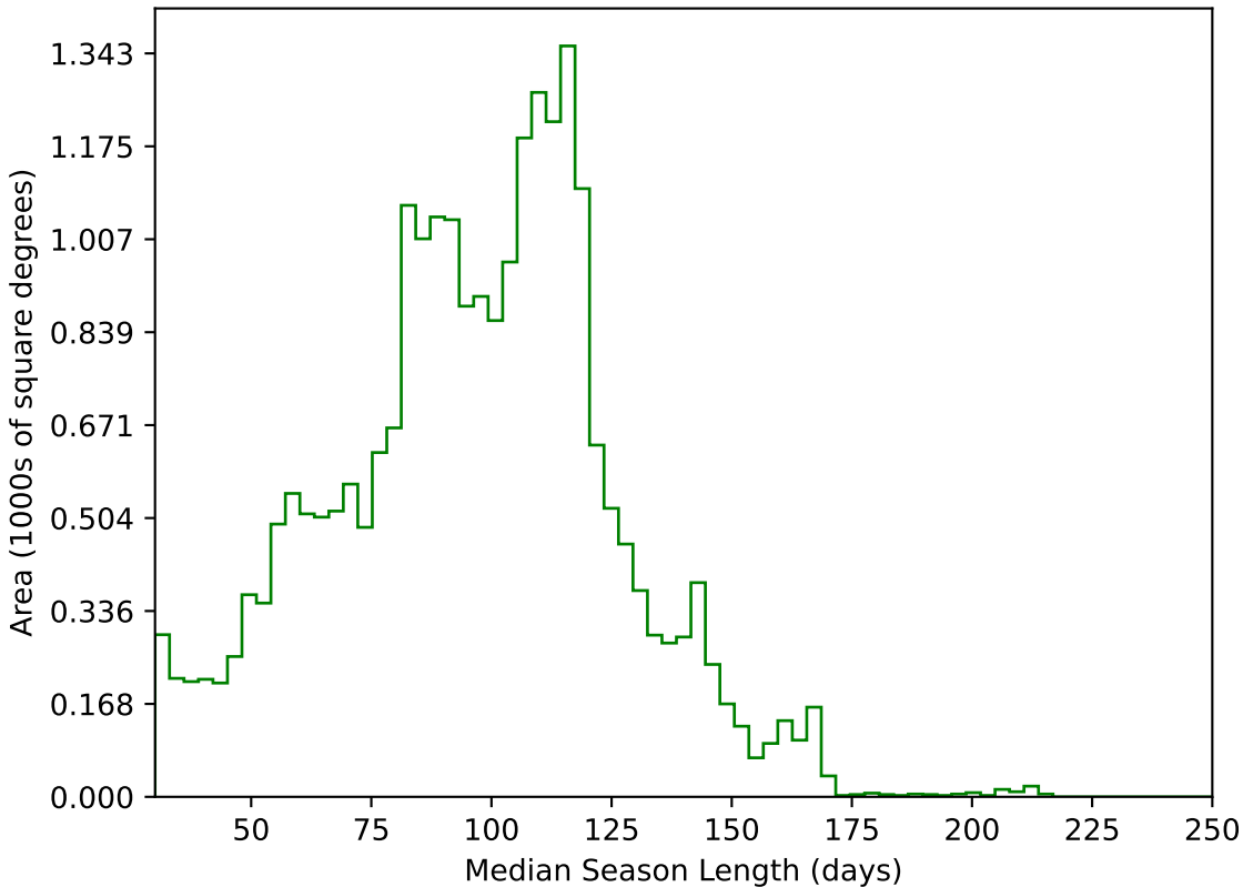
roman_v3.3_10yrs All sky g band: Median Season Length
