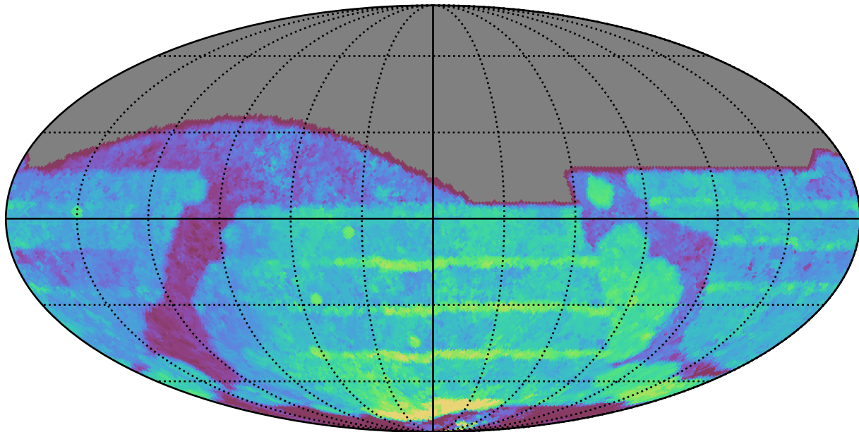
roman_v3.3_10yrs All sky all bands: Median Season Length
