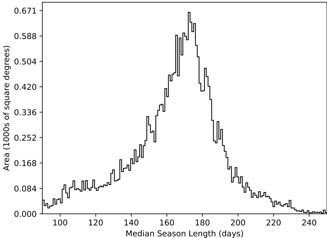
roman_v3.3_10yrs All sky all bands: Median Season Length
