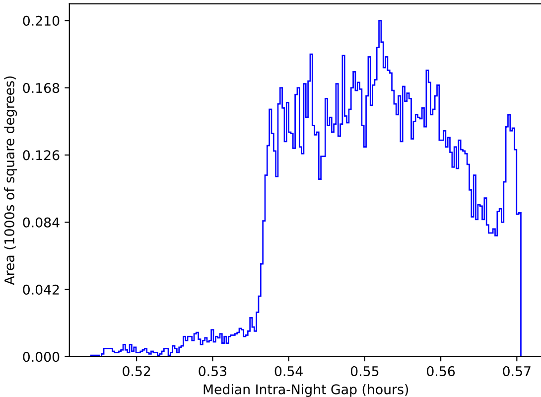
roman_v3.3_10yrs WFD: Median Intra-Night Gap
