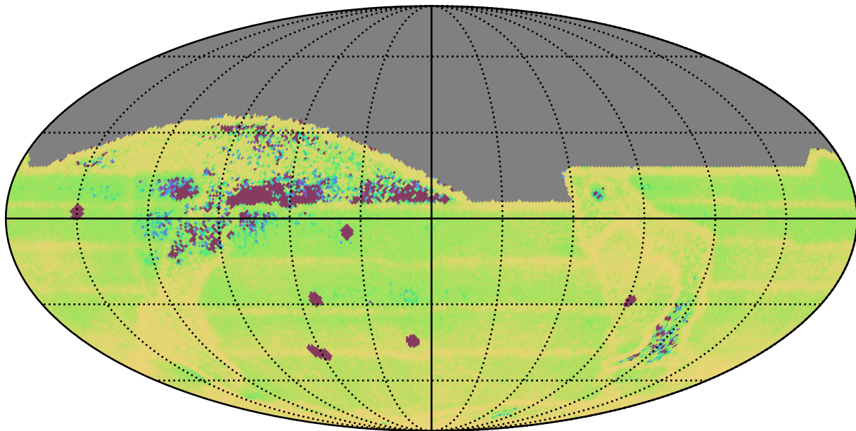
roman_v3.3_10yrs All sky: Median Intra-Night Gap
