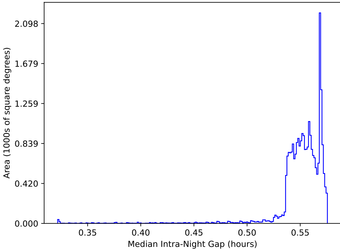
roman_v3.3_10yrs All sky: Median Intra-Night Gap
