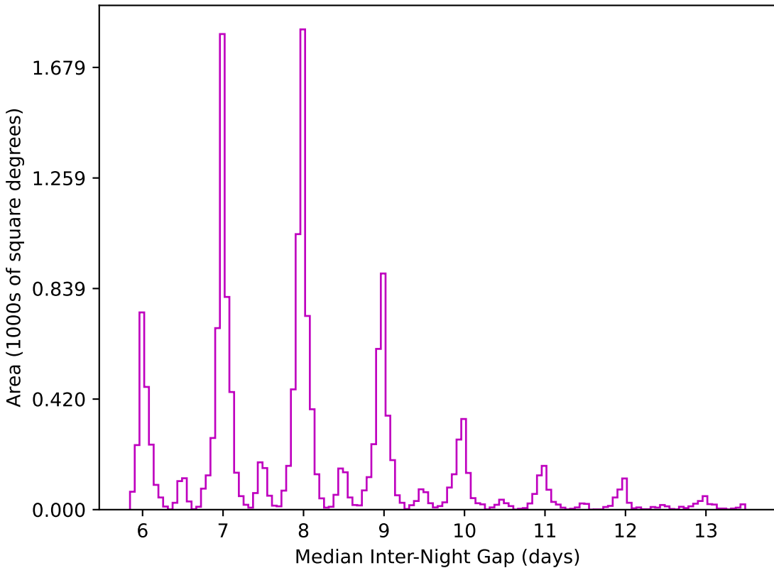
roman_v3.3_10yrs WFD z band: Median Inter-Night Gap
