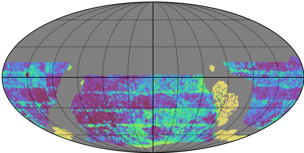
roman_v3.3_10yrs WFD y band: Median Inter-Night Gap
