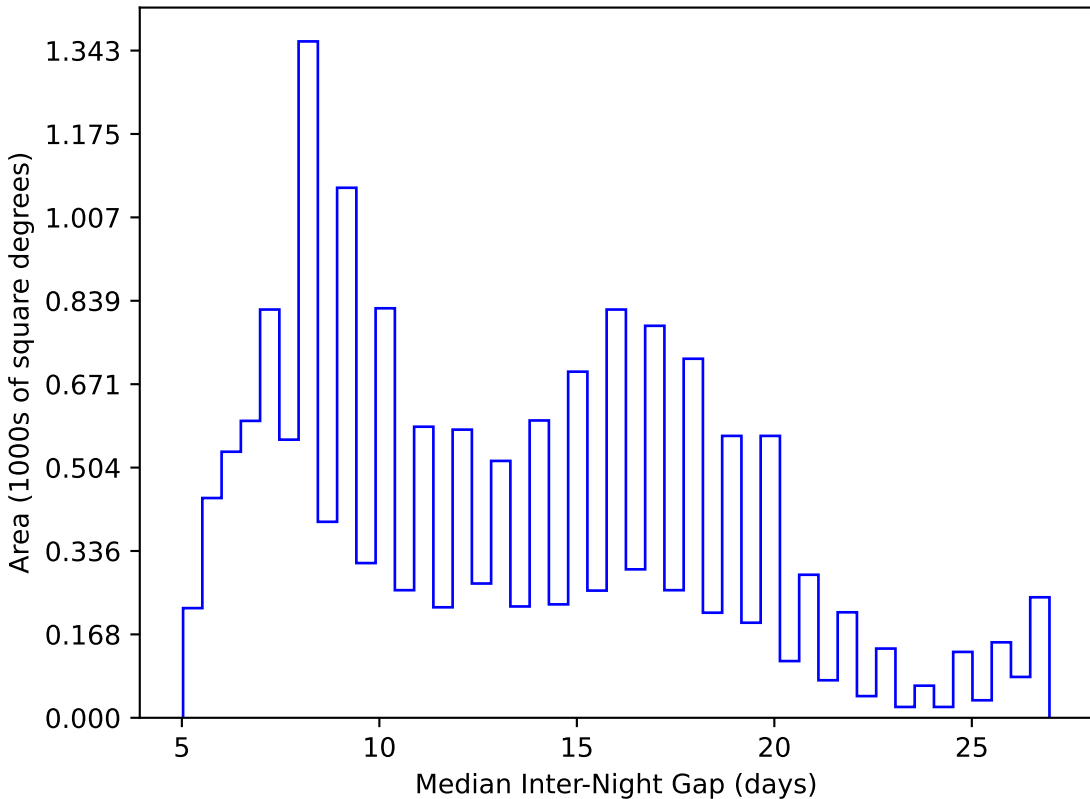
roman_v3.3_10yrs WFD y band: Median Inter-Night Gap
