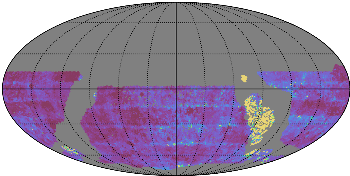
roman_v3.3_10yrs WFD u band: Median Inter-Night Gap
