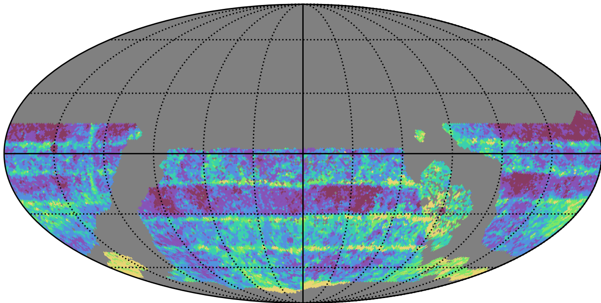
roman_v3.3_10yrs WFD r band: Median Inter-Night Gap
