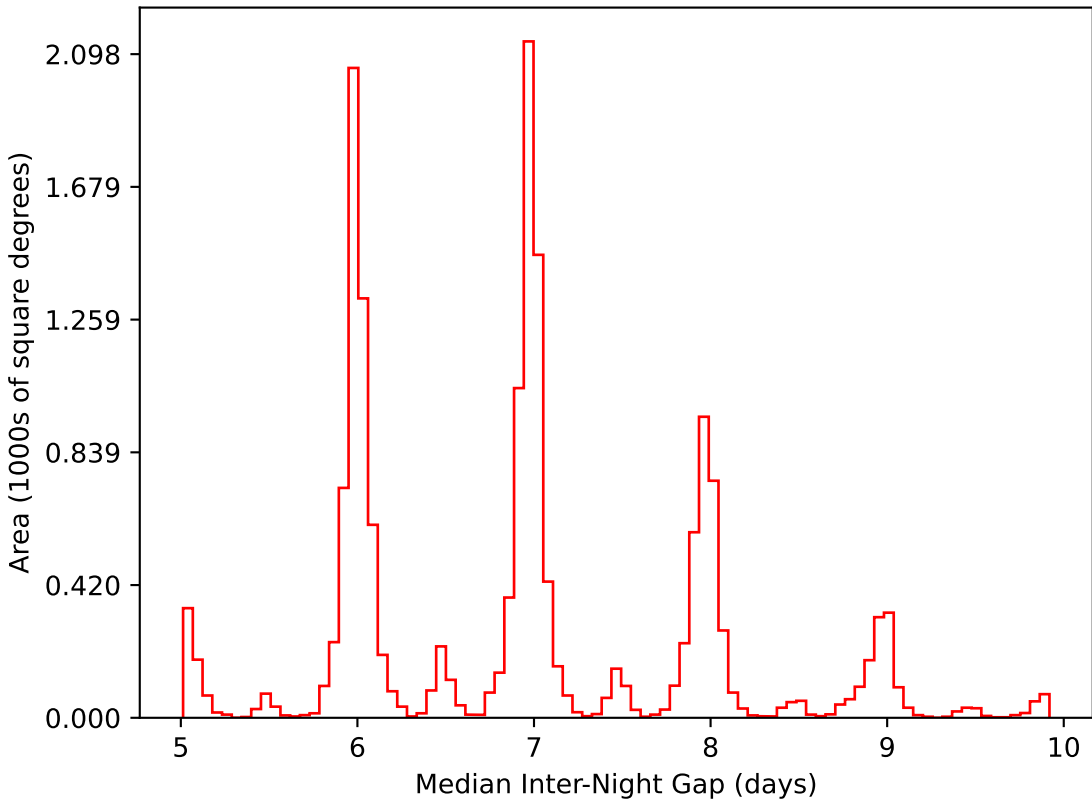
roman_v3.3_10yrs WFD i band: Median Inter-Night Gap
