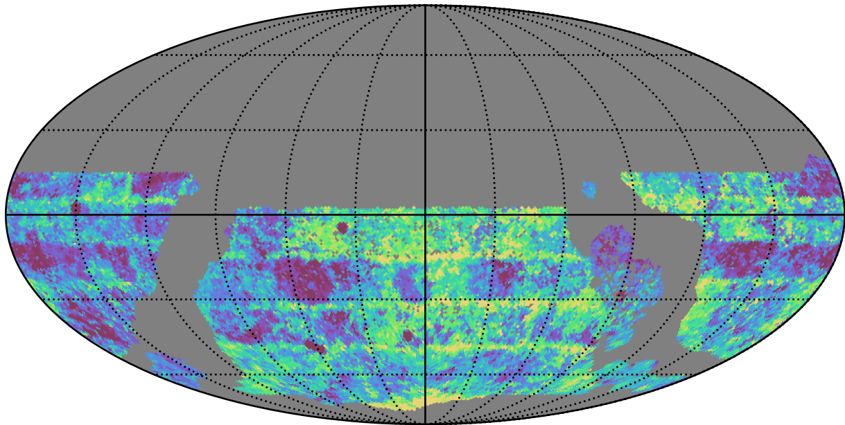
roman_v3.3_10yrs WFD g band: Median Inter-Night Gap
