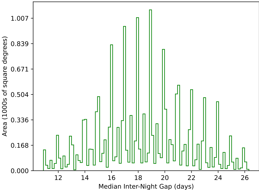
roman_v3.3_10yrs WFD g band: Median Inter-Night Gap
