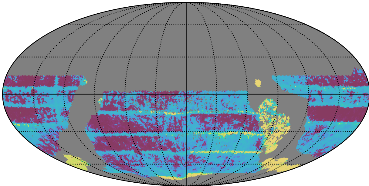
roman_v3.3_10yrs WFD all bands: Median Inter-Night Gap
