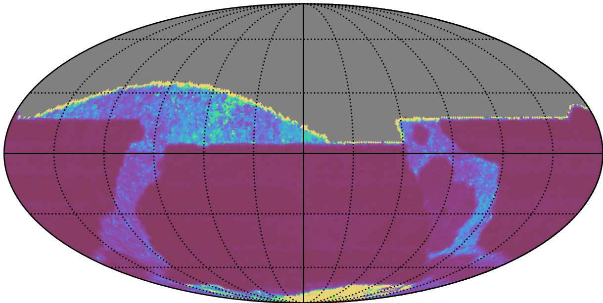
roman_v3.3_10yrs All sky z band: Median Inter-Night Gap
