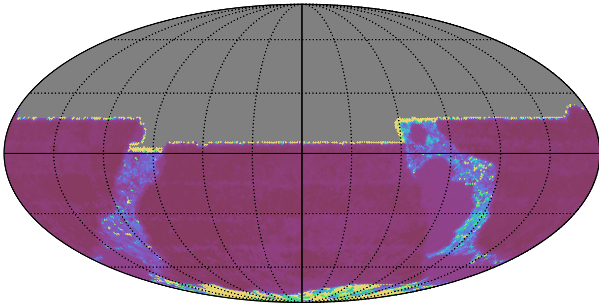
roman_v3.3_10yrs All sky y band: Median Inter-Night Gap
