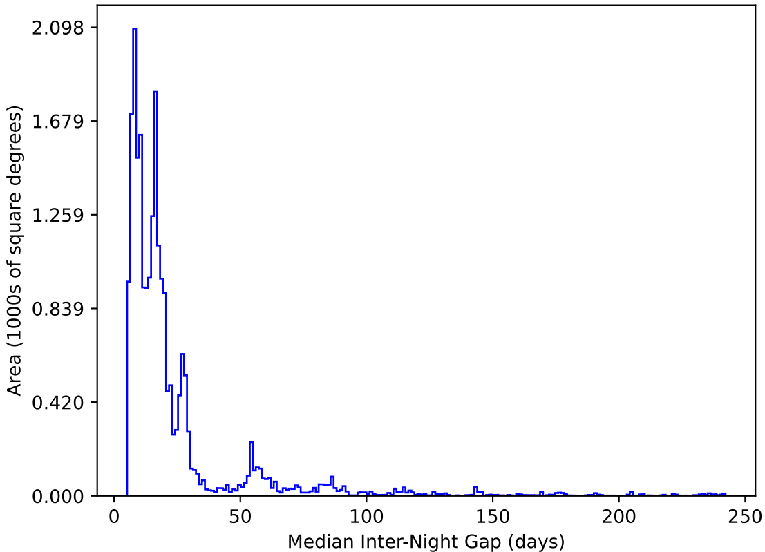
roman_v3.3_10yrs All sky y band: Median Inter-Night Gap
