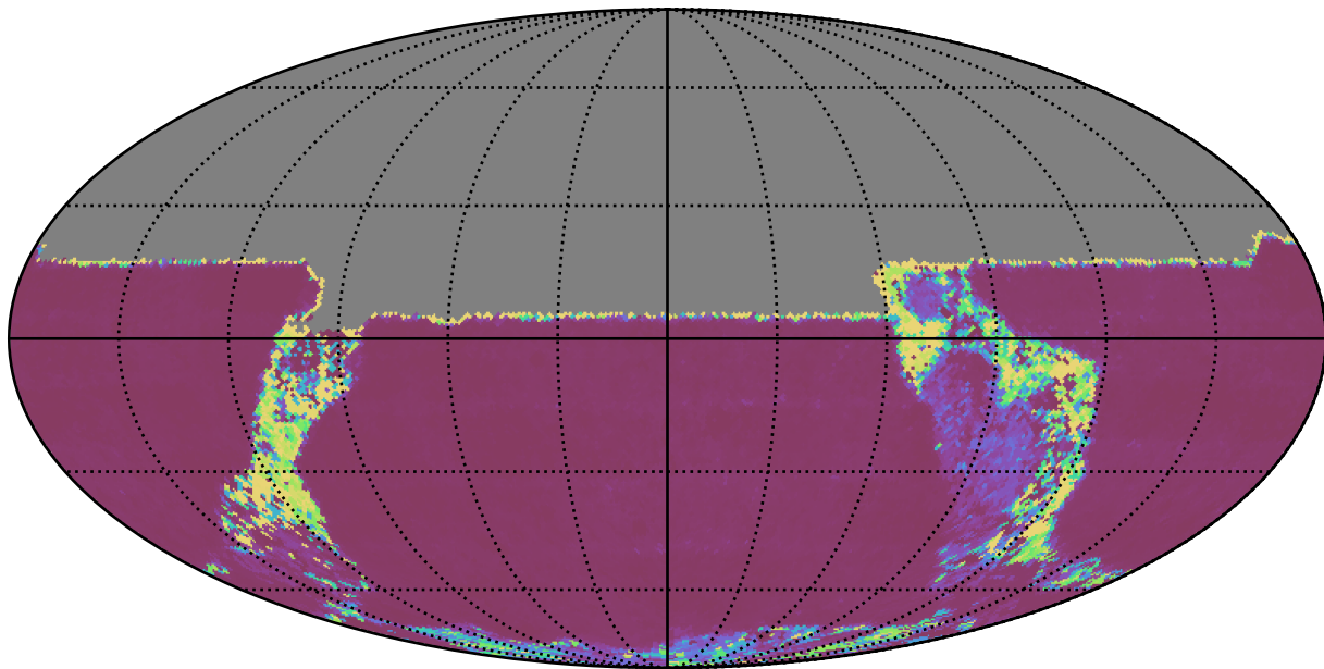
roman_v3.3_10yrs All sky u band: Median Inter-Night Gap
