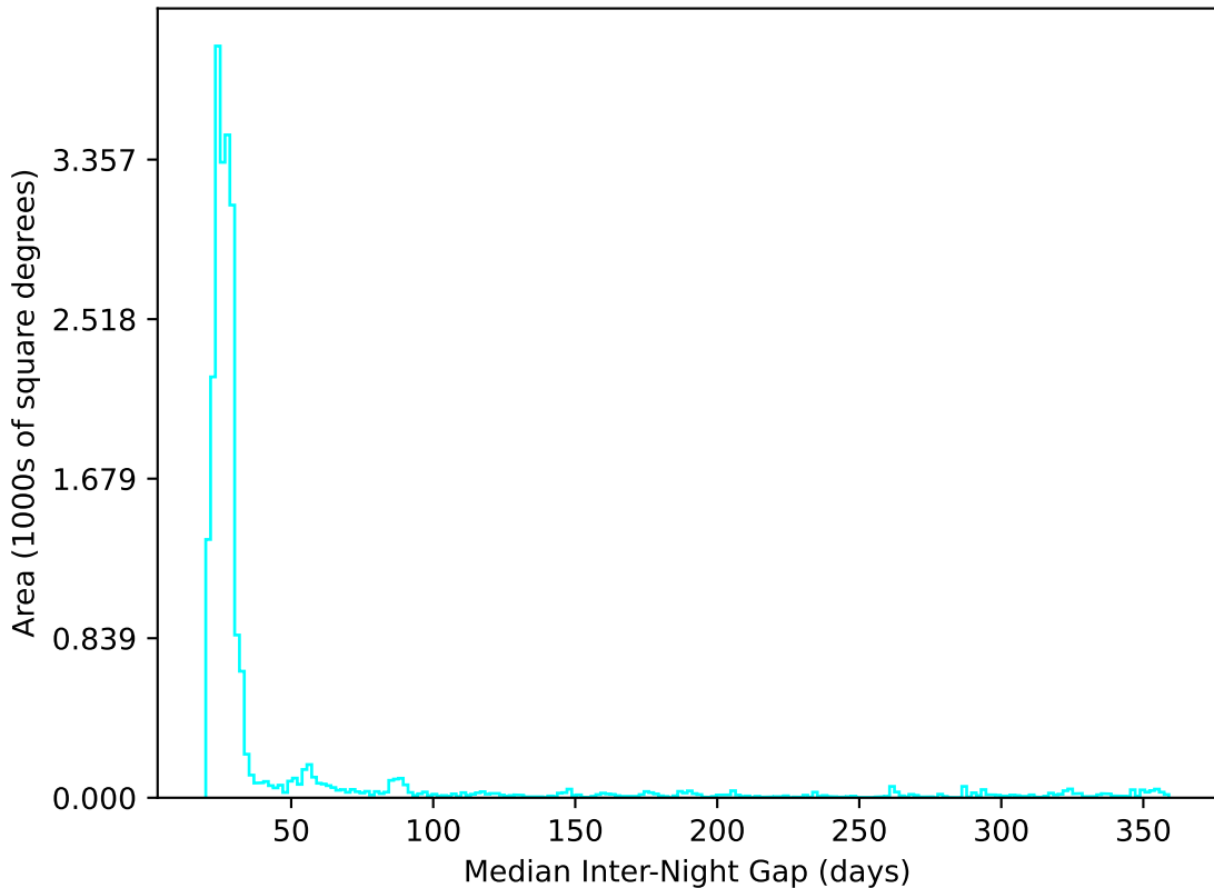
roman_v3.3_10yrs All sky u band: Median Inter-Night Gap
