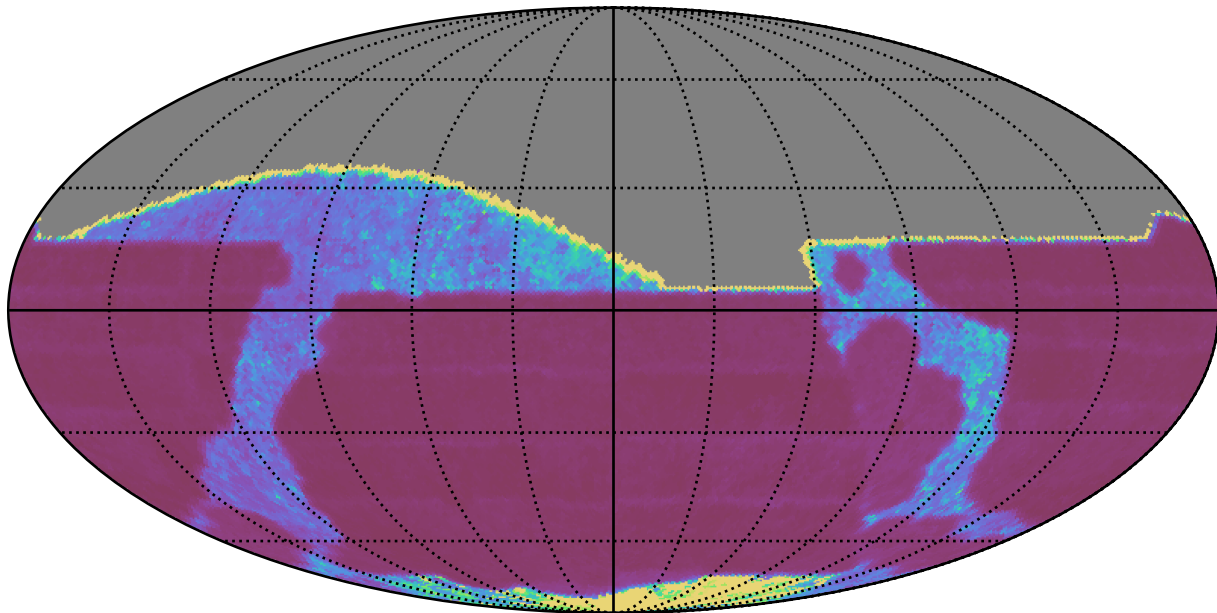
roman_v3.3_10yrs All sky i band: Median Inter-Night Gap
