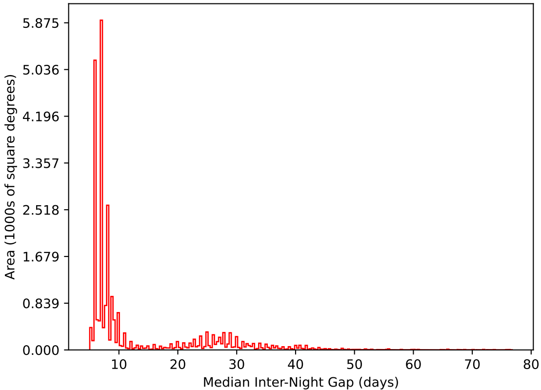
roman_v3.3_10yrs All sky i band: Median Inter-Night Gap
