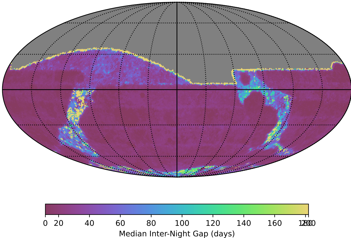
roman_v3.3_10yrs All sky g band: Median Inter-Night Gap
