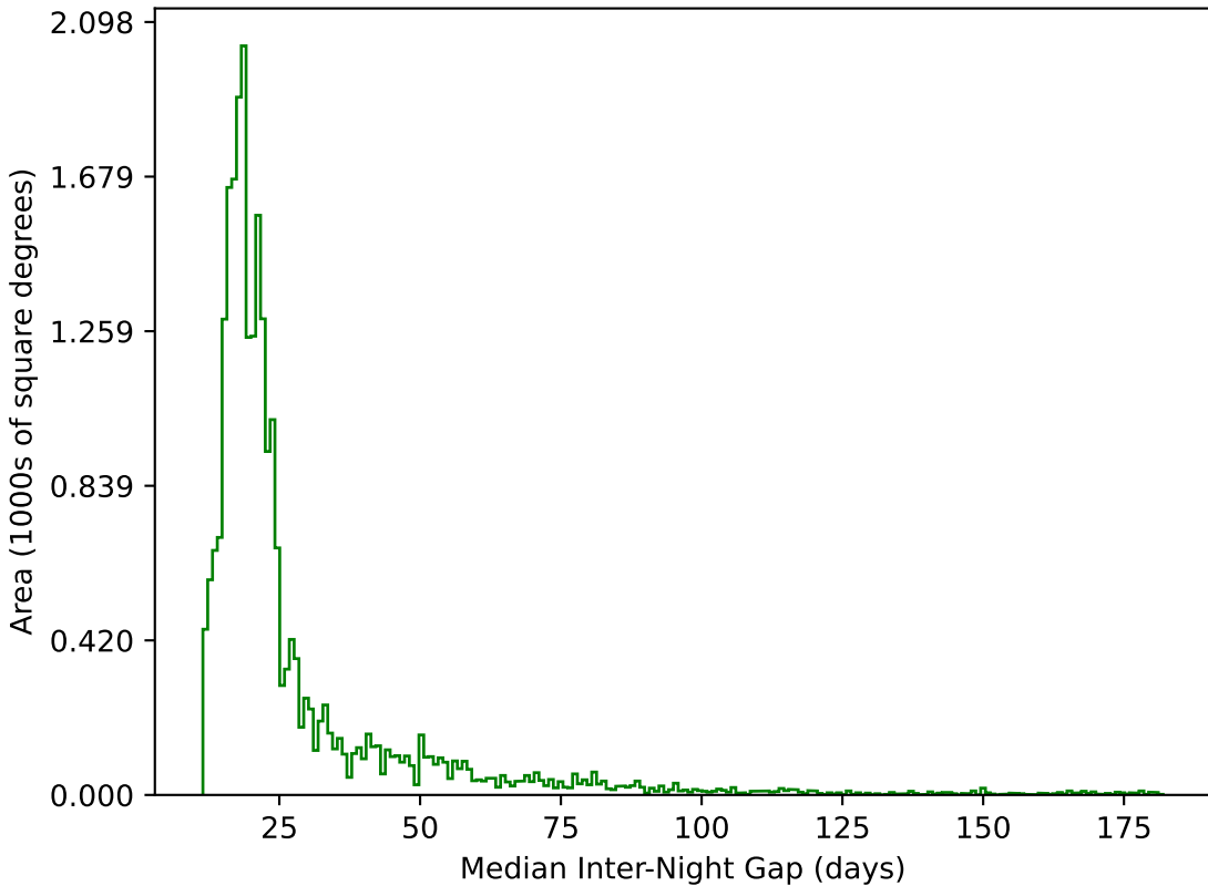
roman_v3.3_10yrs All sky g band: Median Inter-Night Gap
