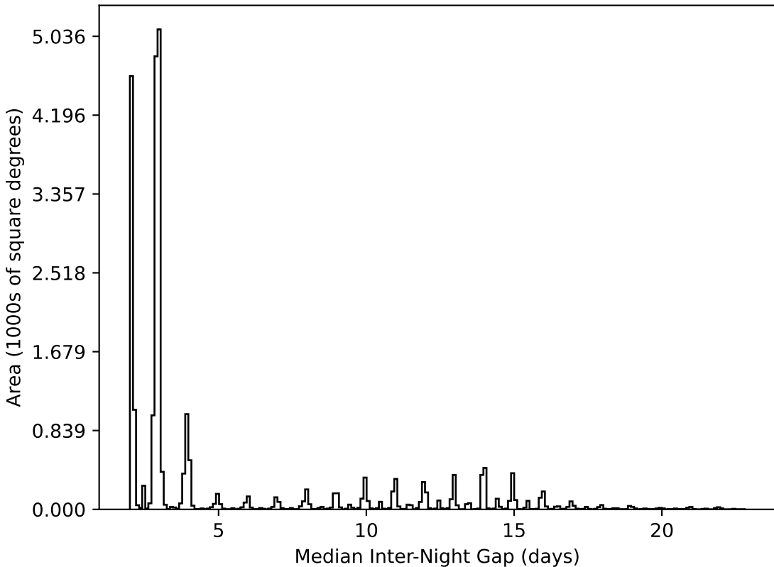
roman_v3.3_10yrs All sky all bands: Median Inter-Night Gap
