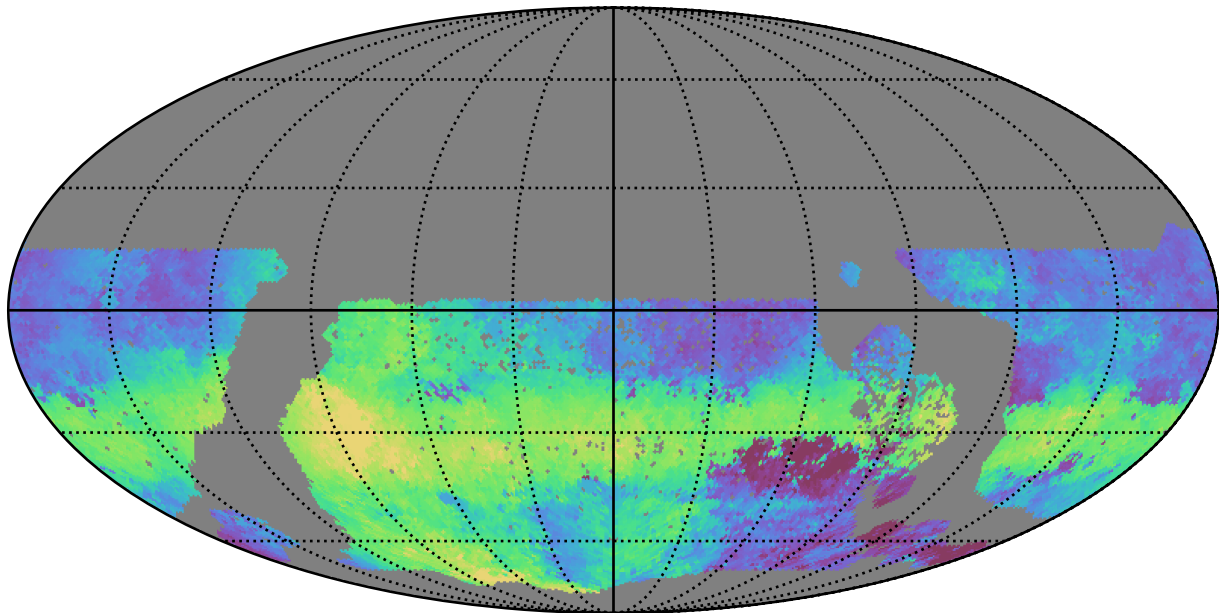
roman_v3.3_10yrs WFD u band: Median HA
