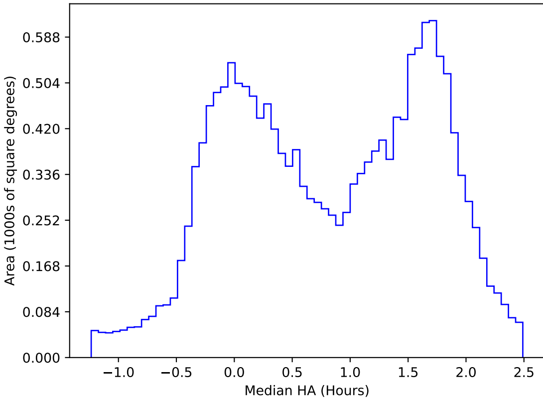
roman_v3.3_10yrs WFD u band: Median HA
